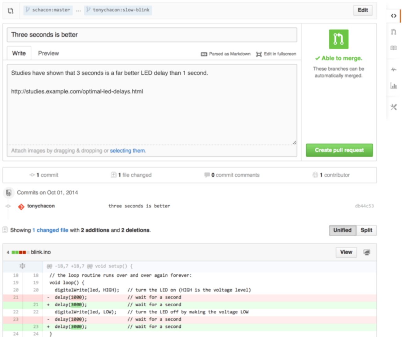
Figure 92. Pull Request creation page
