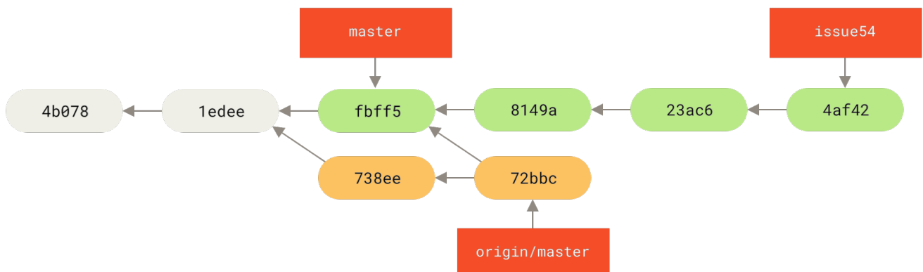
Figure 62. Jessica's history after fetching John's changes.
